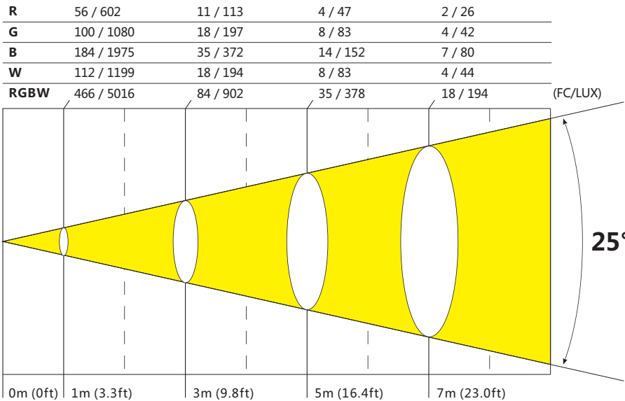
Photometric Beam Angle Data 25° Beam Angle LUX × 0.0929=FC
